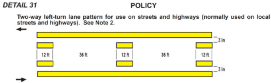
Figure 3A-108 (CA). Two-Way Left-Turn Lanes
